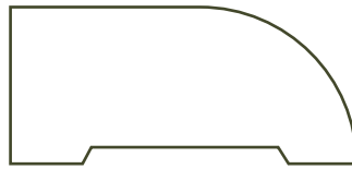
42 x 19 BULLNOSE ARCHITRAVE
